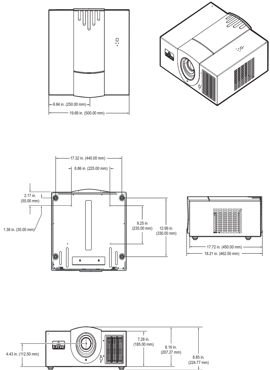
Figure 7-1. CL-810 Dimensions
